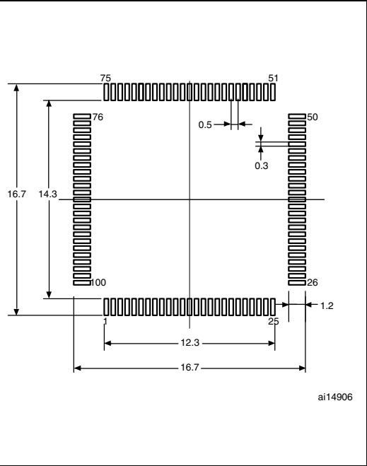
Figure 35. Recommended footprint (1)(2)
