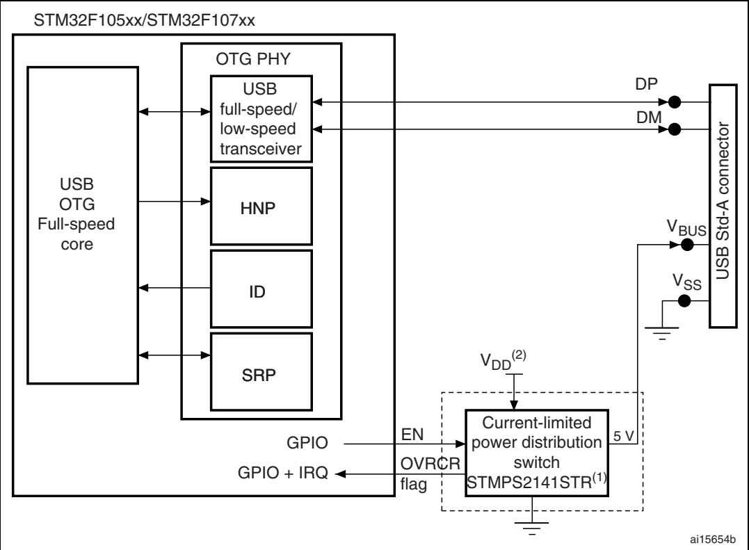
Figure 40. Host connection
