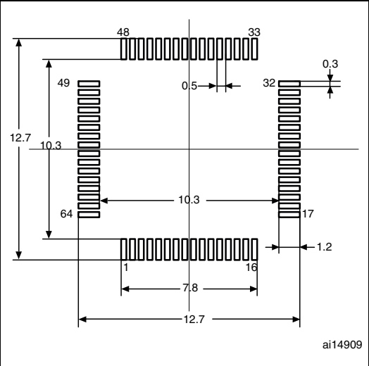
Figure 37. Recommended footprint (1)(2)
