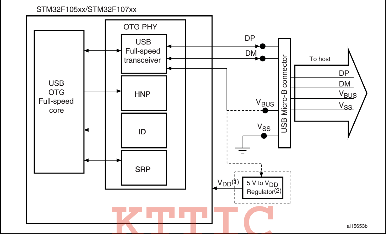
Figure 39. USB OTG FS device mode
