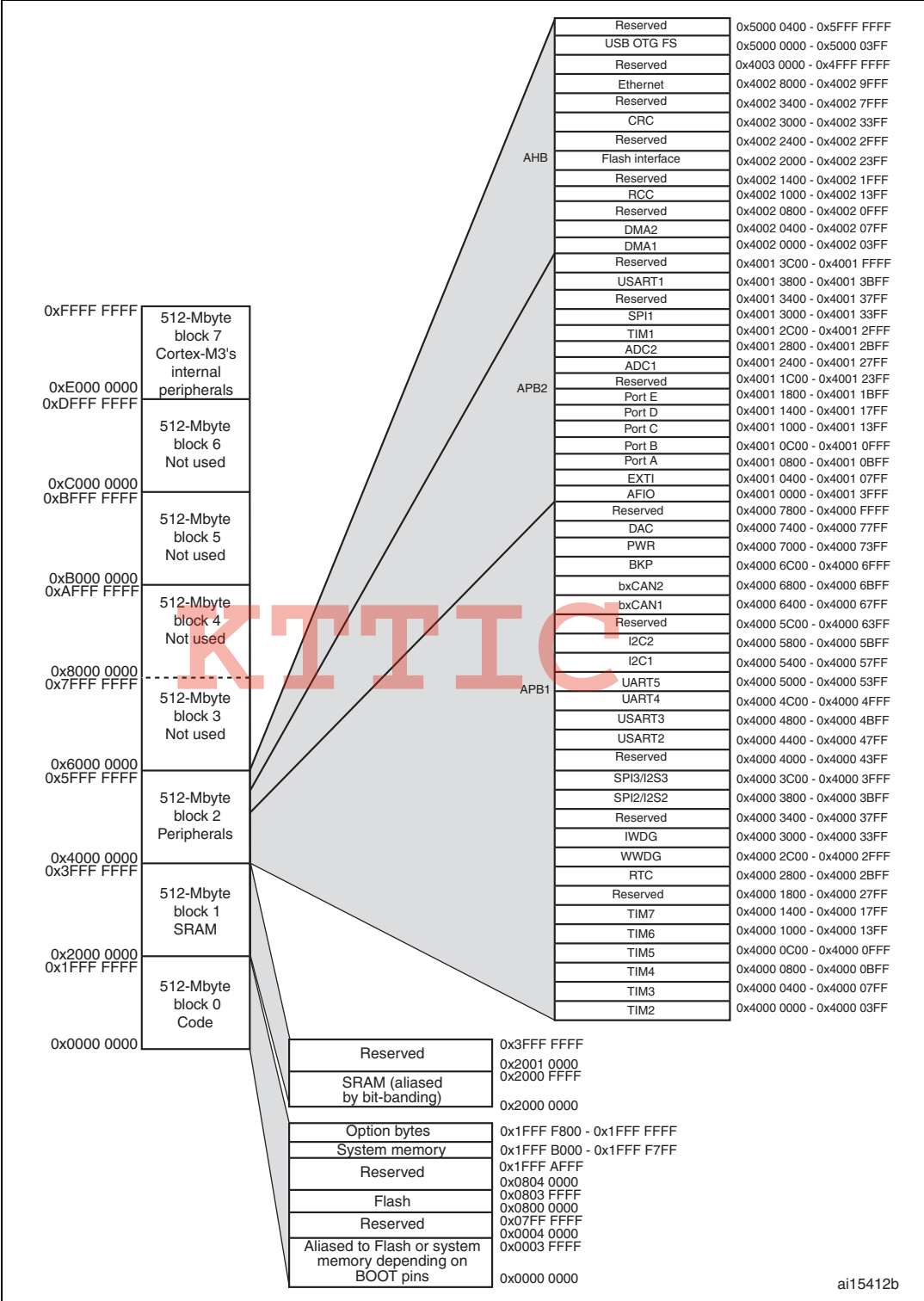
Figure 4. Memory map
