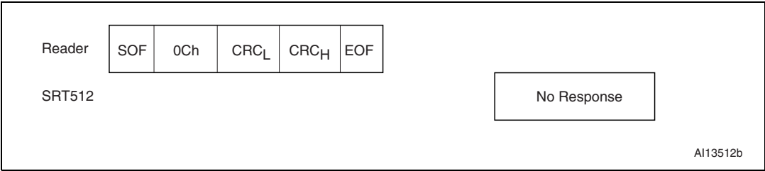
Figure 56. Reset_to_inventory frame exchange between reader and SRT512
