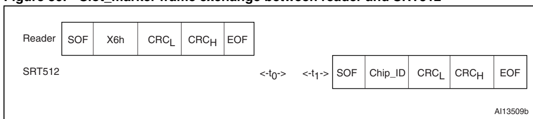
Figure 30. Slot_marker frame exchange between reader and SRT512
