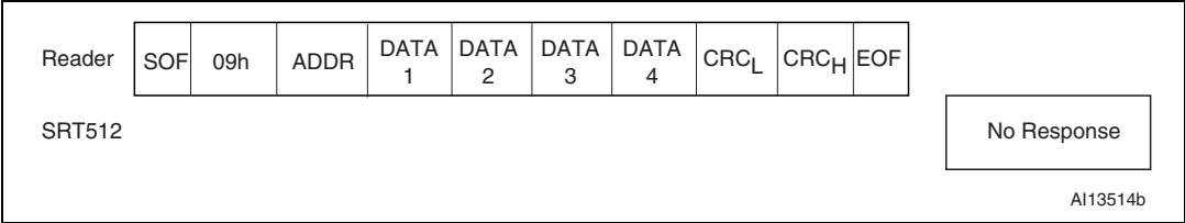
Figure 58. Write_block frame exchange between reader and SRT512
