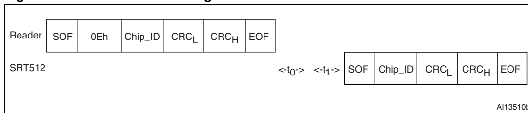
Figure 33. Select frame exchange between reader and SRT512
