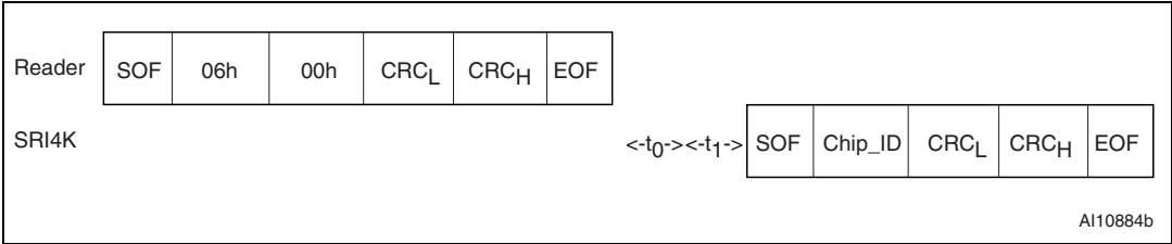
Figure 52. Initiate frame exchange between reader and SRI4K
