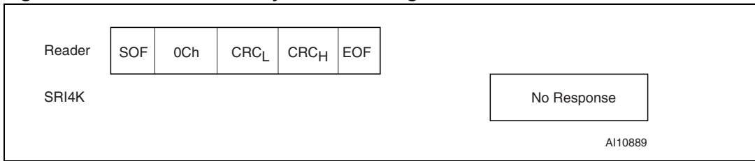
Figure 57. Reset_to_inventory frame exchange between reader and SRI4K
