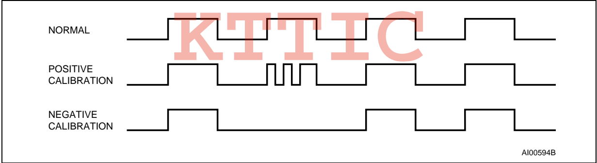
Figure 11. Calibration Waveform
