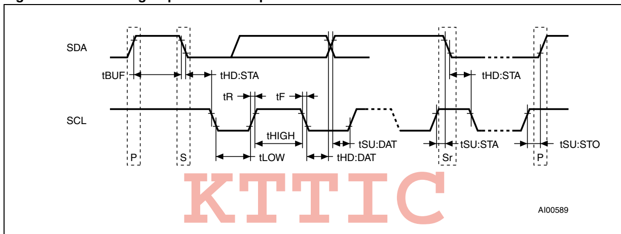
Figure 14. Bus timing requirements sequence
