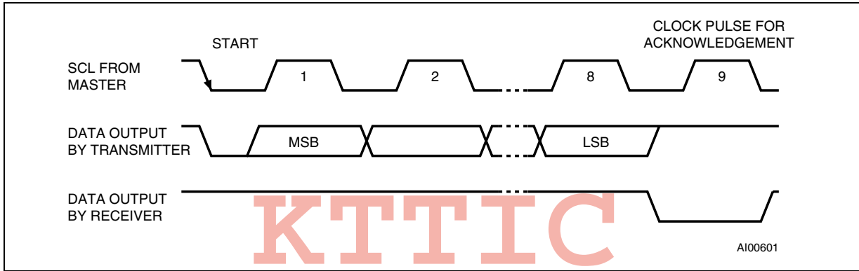
Figure 5. Acknowledgement sequence
