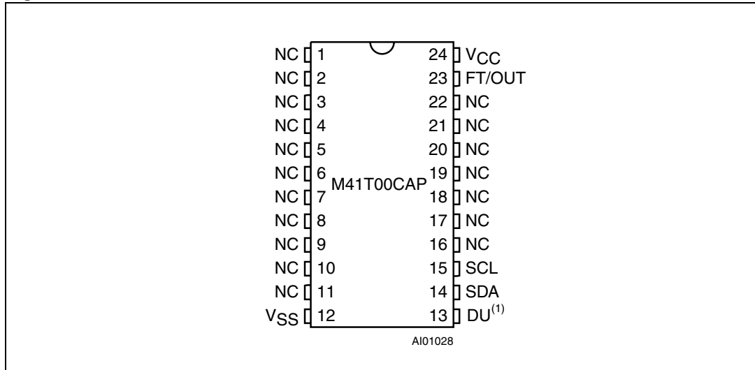
Figure 2. DIP connections
