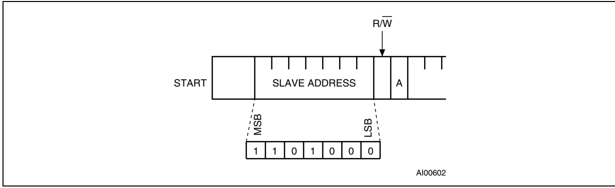
Figure 7. READ mode sequence
