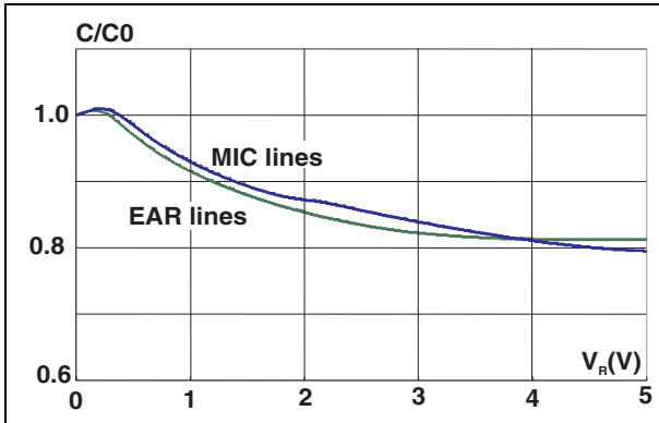
Figure 10. Relative line capacitance variation versus applied voltage
