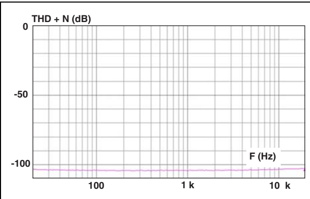
Figure 11. Total harmonic distortion with noise: MIC lines, R = 10 kΩ
