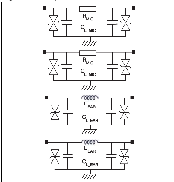
Figure 2. Equivalent circuit
