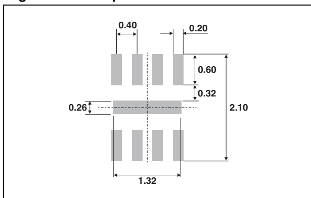
Figure 17. Footprint
