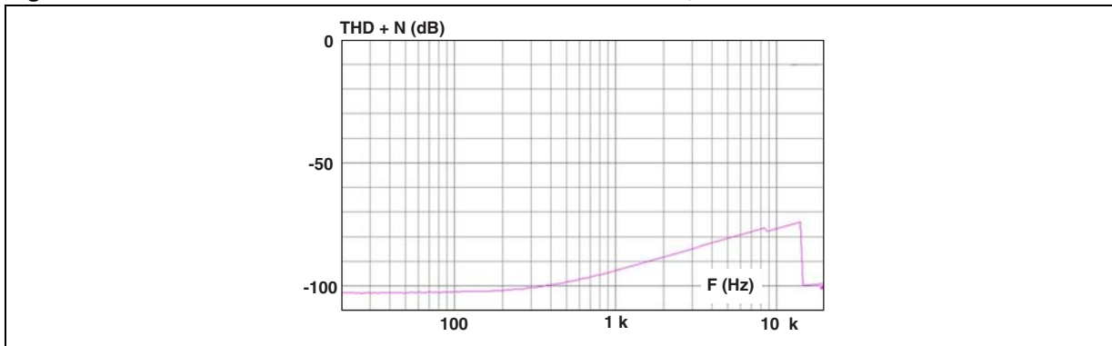
Figure 14. Total harmonic distortion with noise: EAR lines, R = 8 Ω
