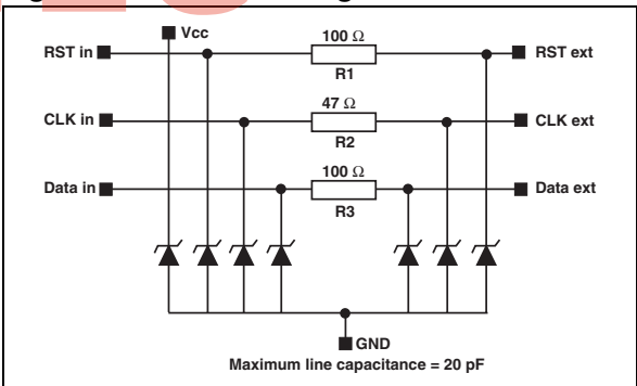
Figure 2. Device configuration
