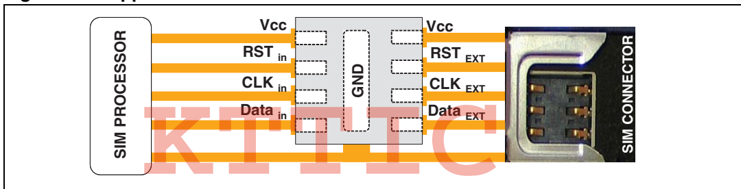
Figure 11. Application schematic
