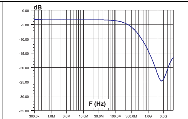
Figure 4. S21(db) attenuation (CLK line)
