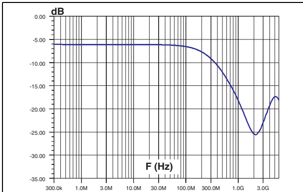
Figure 3. S21(db) attenuation (RST line)
