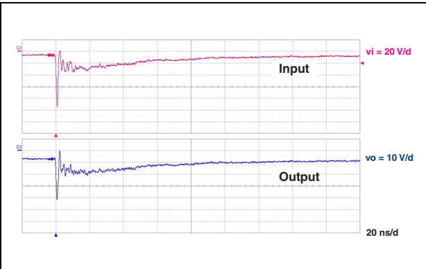
Figure 6. ESD response to IEC 61000-4-2 (-8 kV air discharge) on MIC lines
