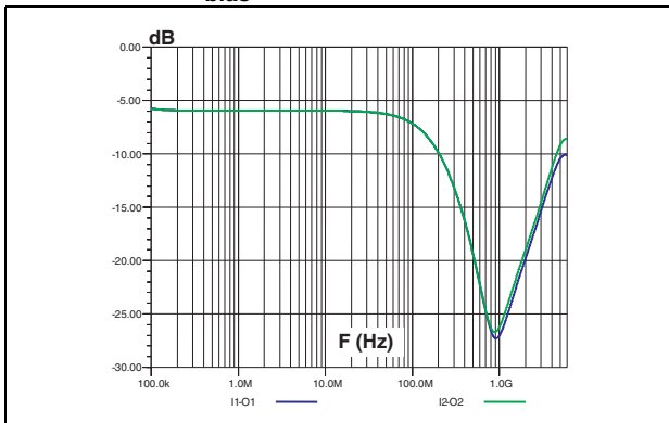
Figure 3. S21(db) attenuation measurement (V bias = 0 V)
