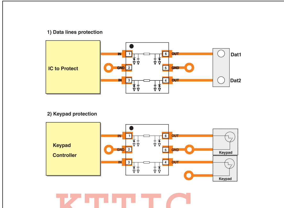
Figure 8. Application schematic
