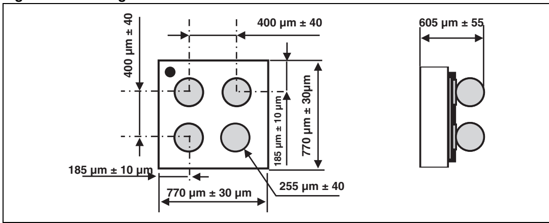
Figure 10. Package dimensions
