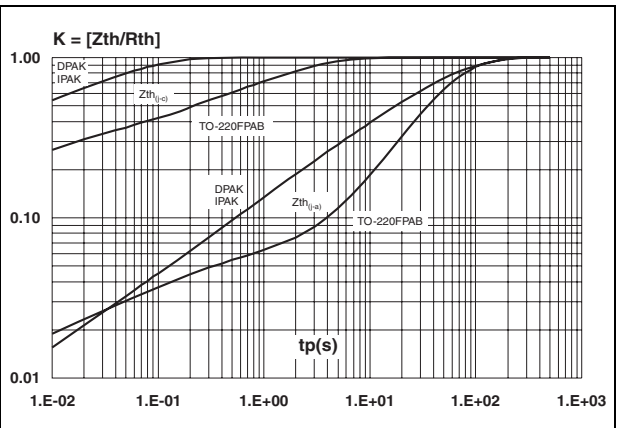
Figure 8. Relative variation of thermal impedance versus pulse duration.
