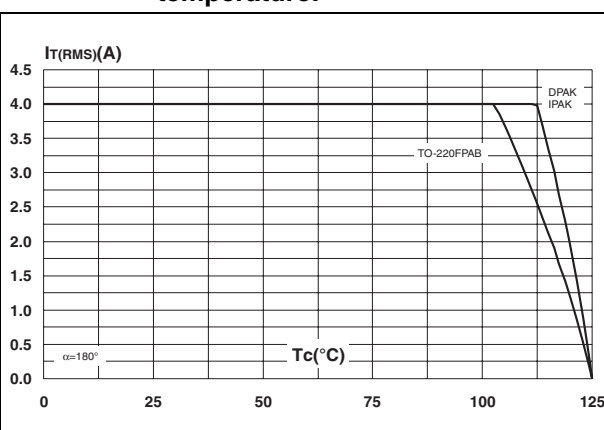
Figure 6. RMS on-state current versus case temperature.
