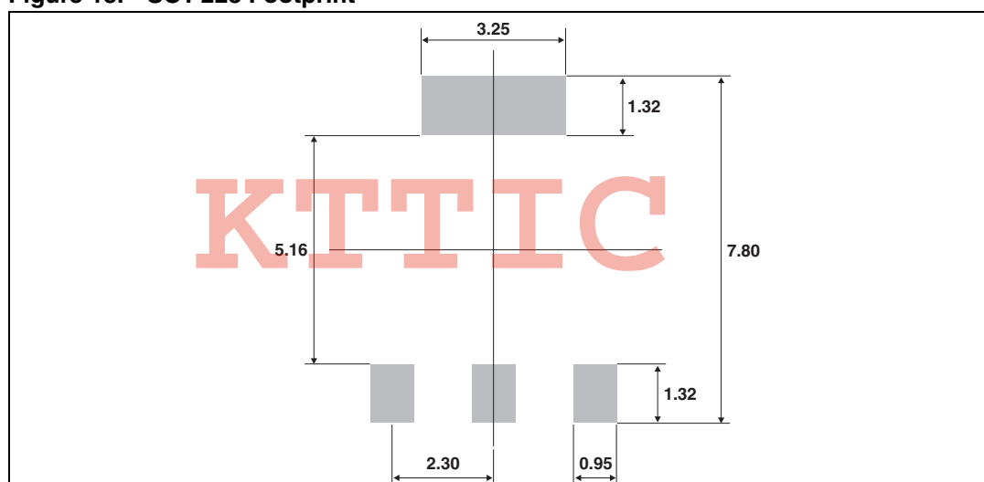
Figure 18. SOT-223 Footprint
