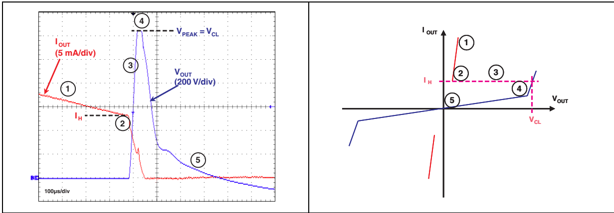
Figure 14. Effect of the switching off of a high inductive load - typical clamping capability of ACS102-6T
