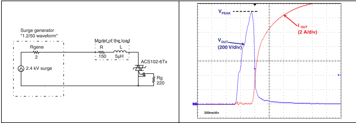
Figure 16. Overvoltage ruggedness test circuit with conditions equivalent to IEC 61000-4-5 standards
