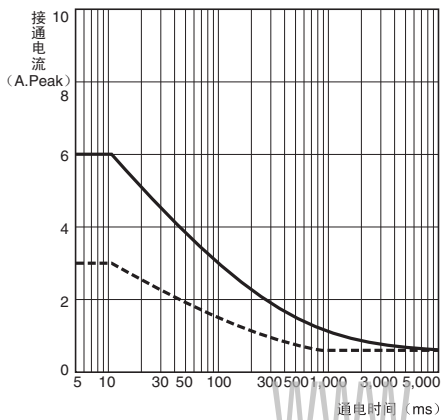
G3DZ-2R6PL
