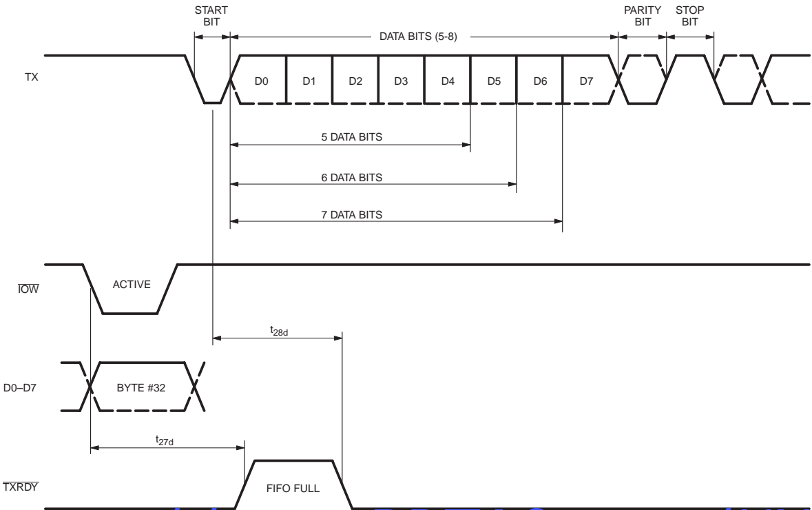
http://www.BDTIC.com/NXP Fig 23. Transmit ready timing in FIFO mode (DMA mode '1').
