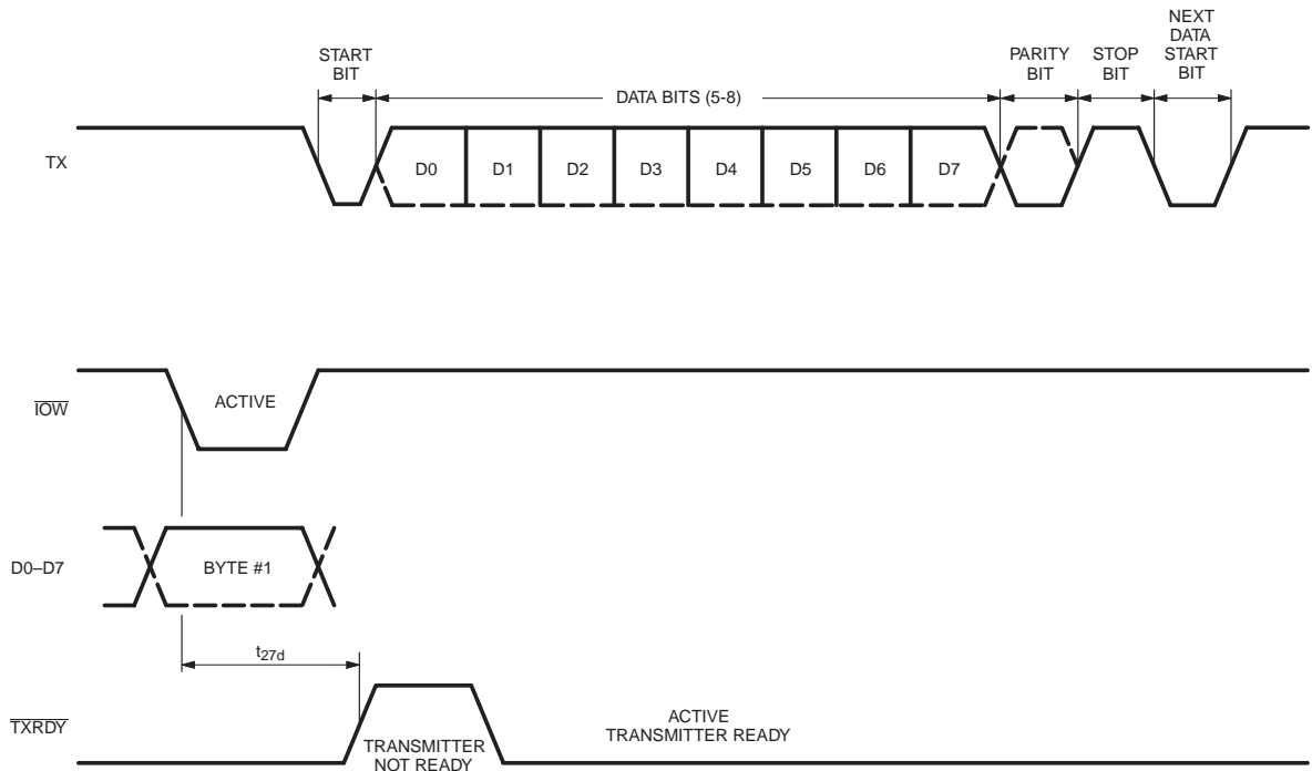
Fig 2. Transmit ready timing in non-FIFO mode.
