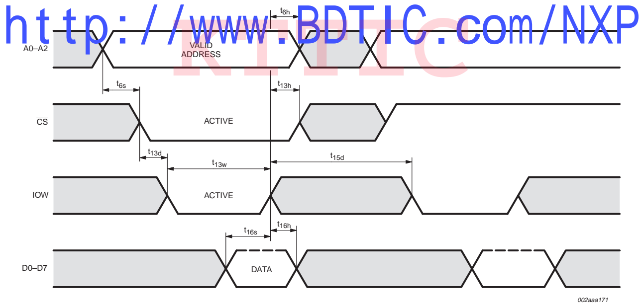
Fig 11. General write timing in 16 mode.
