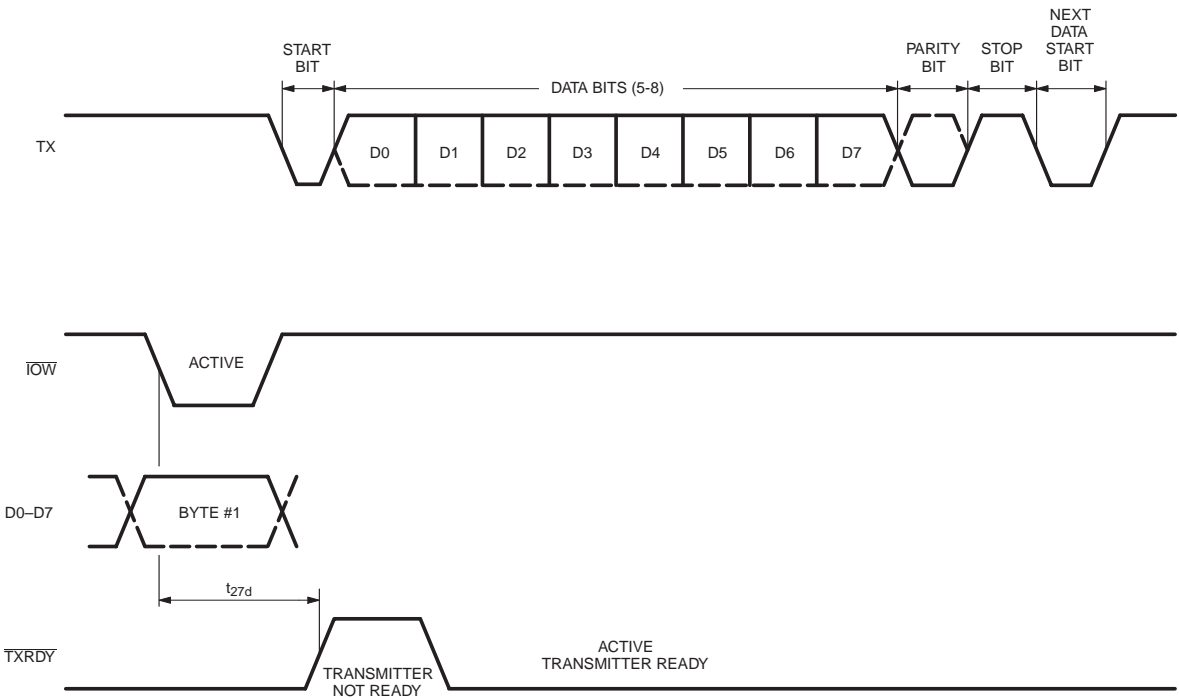
Fig 3. Transmit ready timing in non-FIFO mode.
