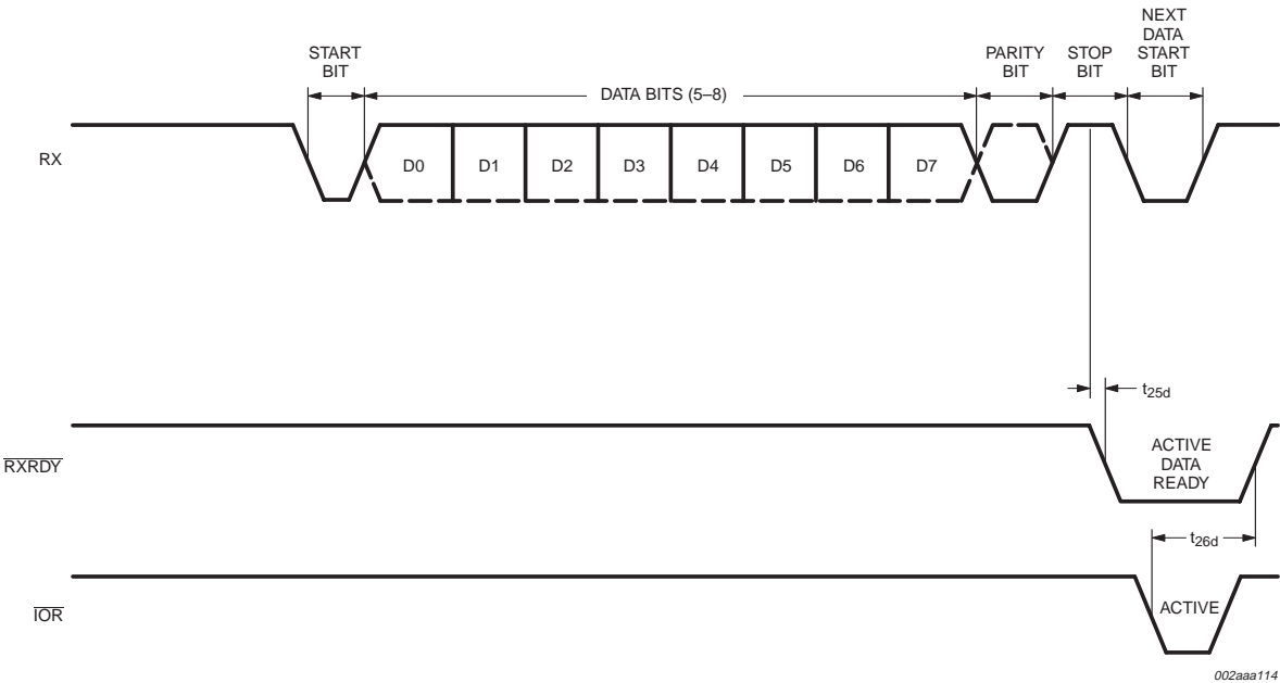
Fig 17. Receive ready timing in non-FIFO mode.
