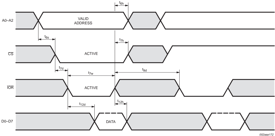
Fig 13. General read timing in 16 mode.
