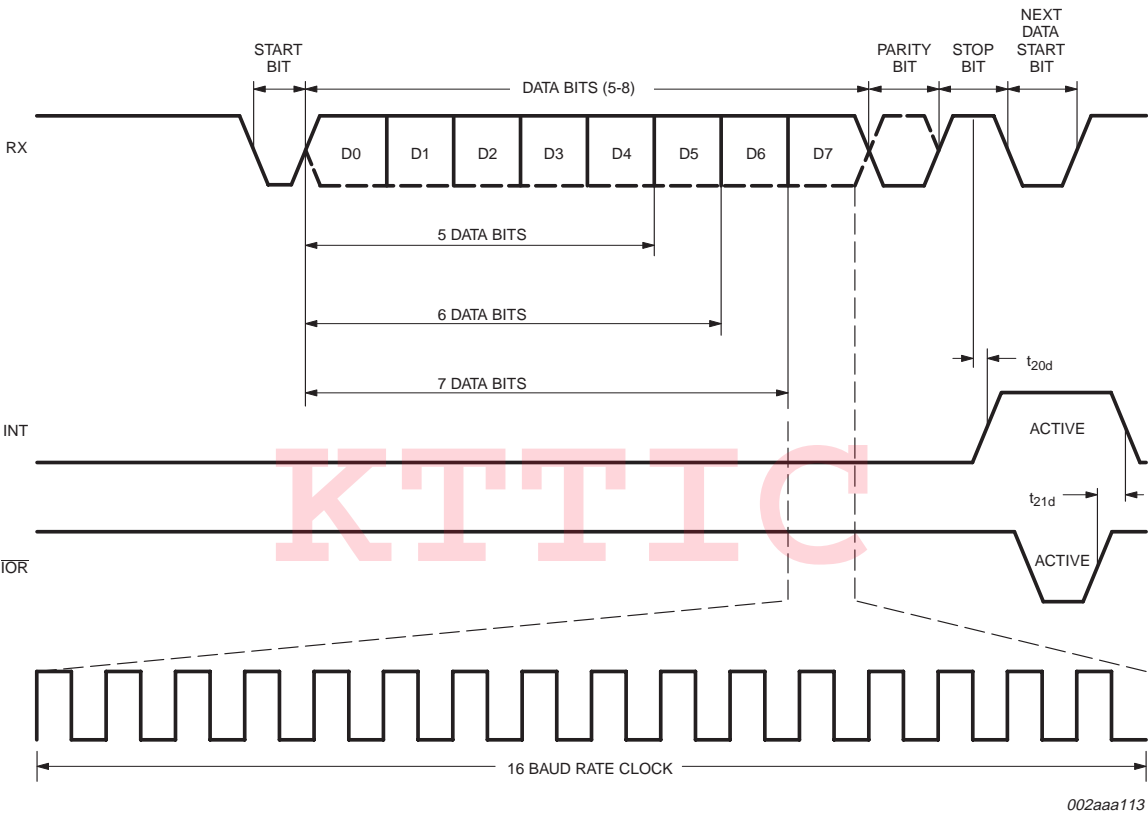
Fig 16. Receive timing.
