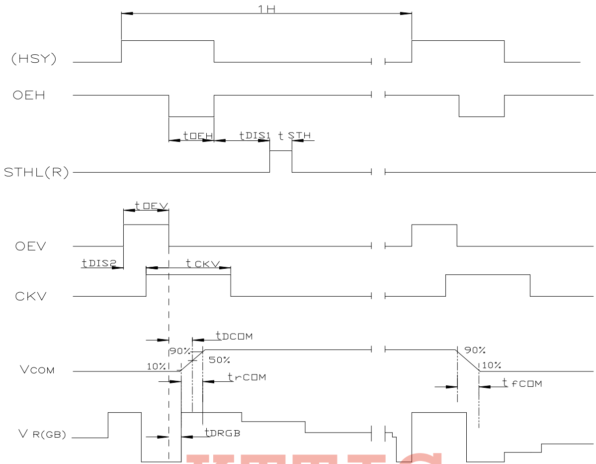
Note: The falling edge of OEV should be synchronized with the falling edge of OEH Fig.3-3-(b) Detail horizontal timing
