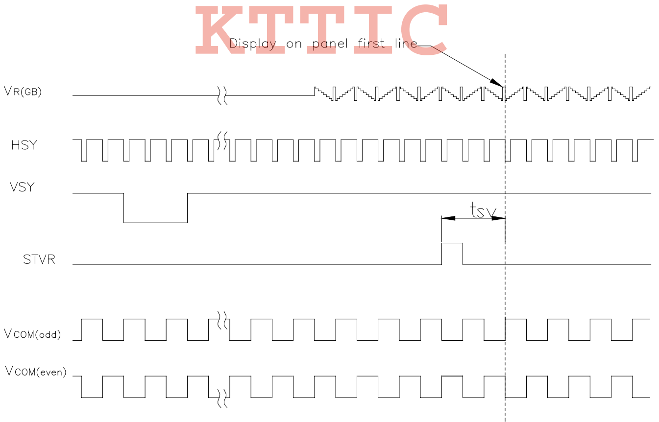
Fig.3-5(b) Vertical timing (from down to up)
