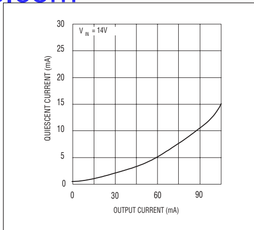
Figure 2. Quiescent Current
