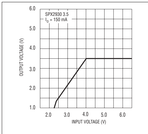
Figure 6. Low Voltage Behavior
