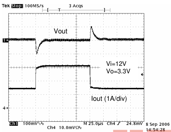
Figure 3. Load Step Response: 1.5->3A
