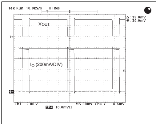
Current Limit
