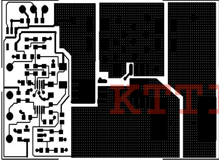
Figure 12. SP6132EB PC Layout Top Side
