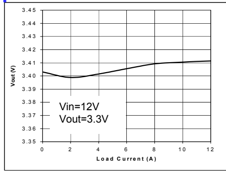
Figure 2. Load Regulation
