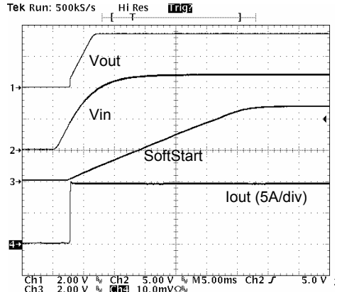
Figure 7. Start-Up Response: 10A Load
