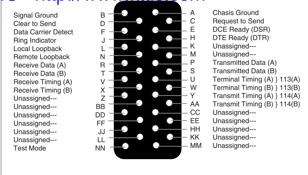
Figure 26. ISO-2593 Connector Pin Out
