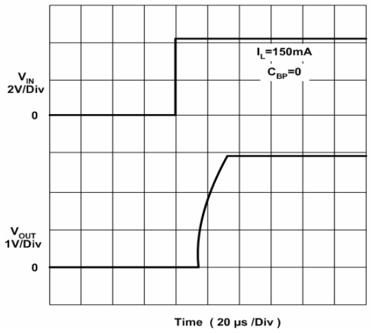
Start Up Time ( V_{IN}=4.2V )
