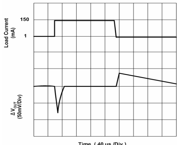
Load Transient Response ( V_{IN}=3.2V )
