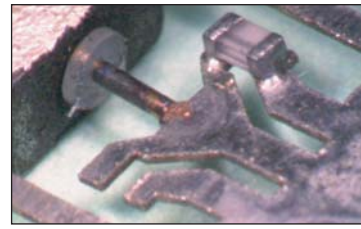
Anode, fuse and leadframe assembly
