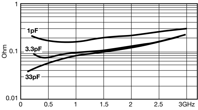
Typical ESR vs. Frequency Accu-F®/Accu-P® 0805
