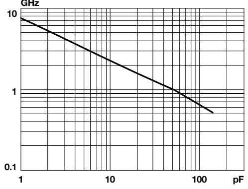
Typical Self Resonant Frequency vs. Capacitance Accu-F®/Accu-P® 0805
