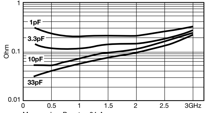
Typical ESR vs. Frequency Accu-P® 1210
