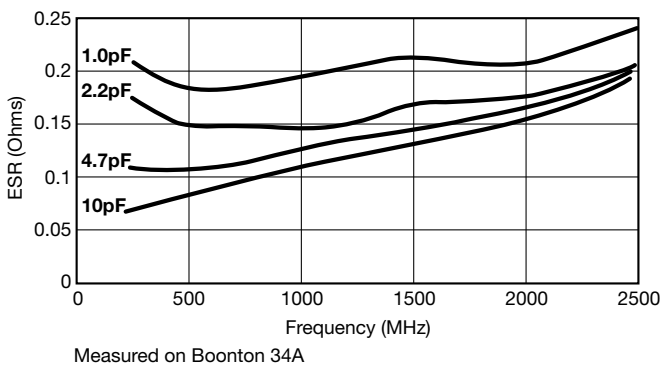
Typical ESR vs. Frequency Accu-P® 0402
