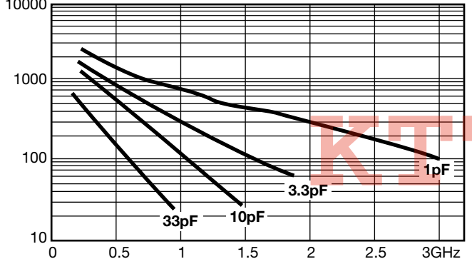
Typical Q vs. Frequency Accu-F®/Accu-P® 0805
