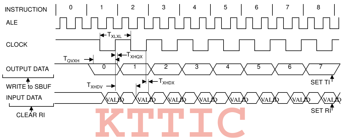
Figure 14-9. Shift Register Timing Waveforms
