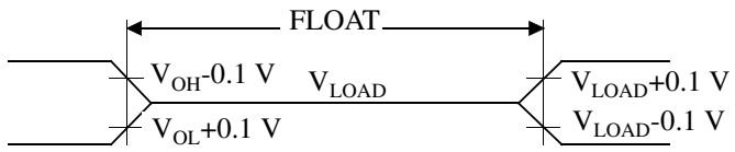
Figure 14-12. Float Waveforms
