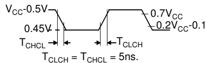
Figure 14-5. Clock Signal Waveform for I_{CC} Tests in Active and Idle Modes
