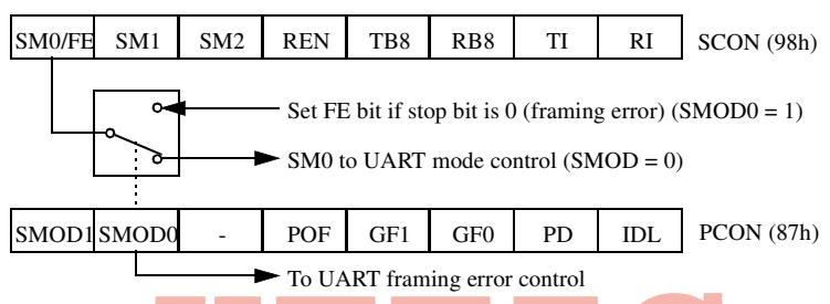
Figure 9-1. Framing Error Block Diagram
