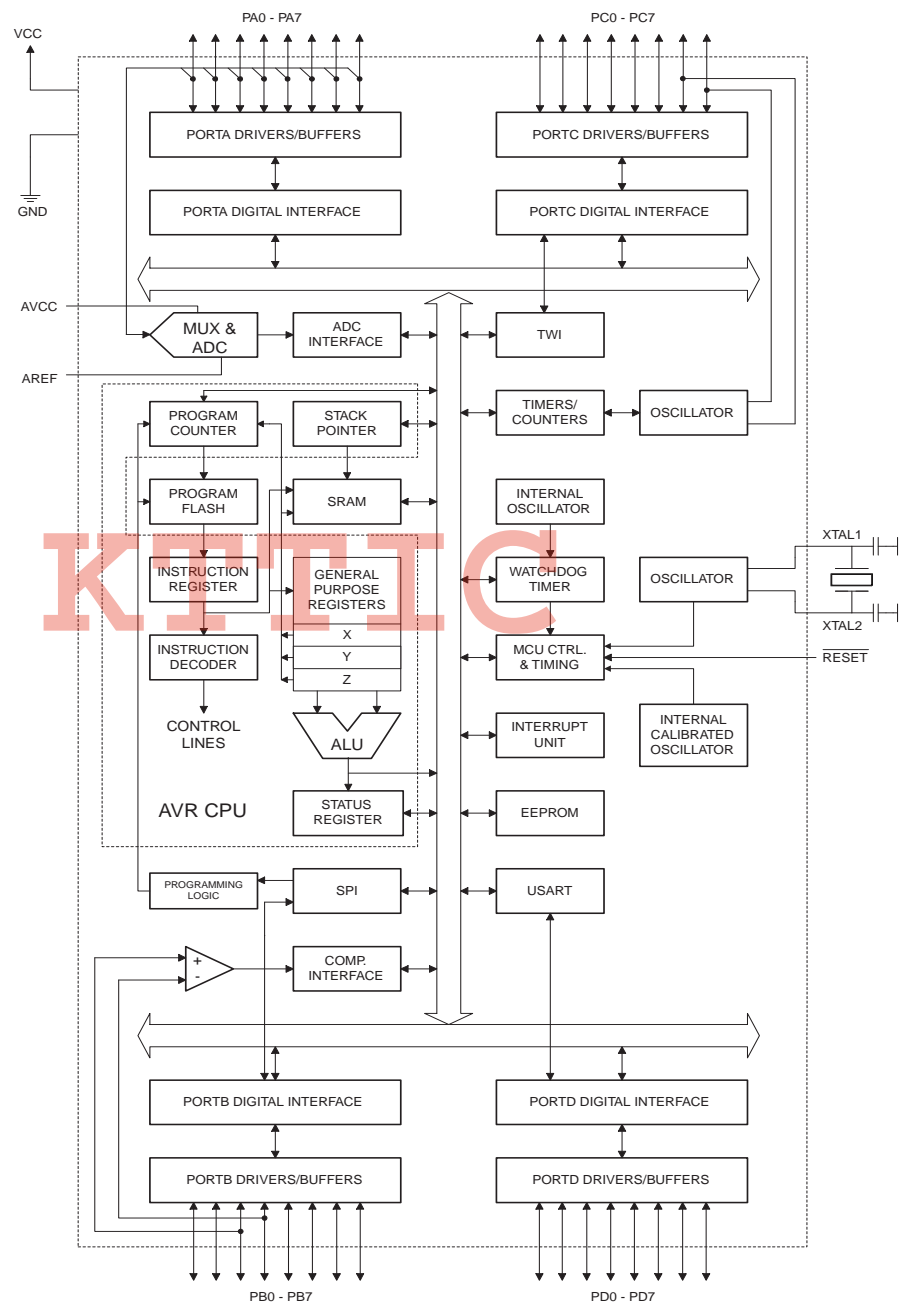
Figure 2-1. Block Diagram
