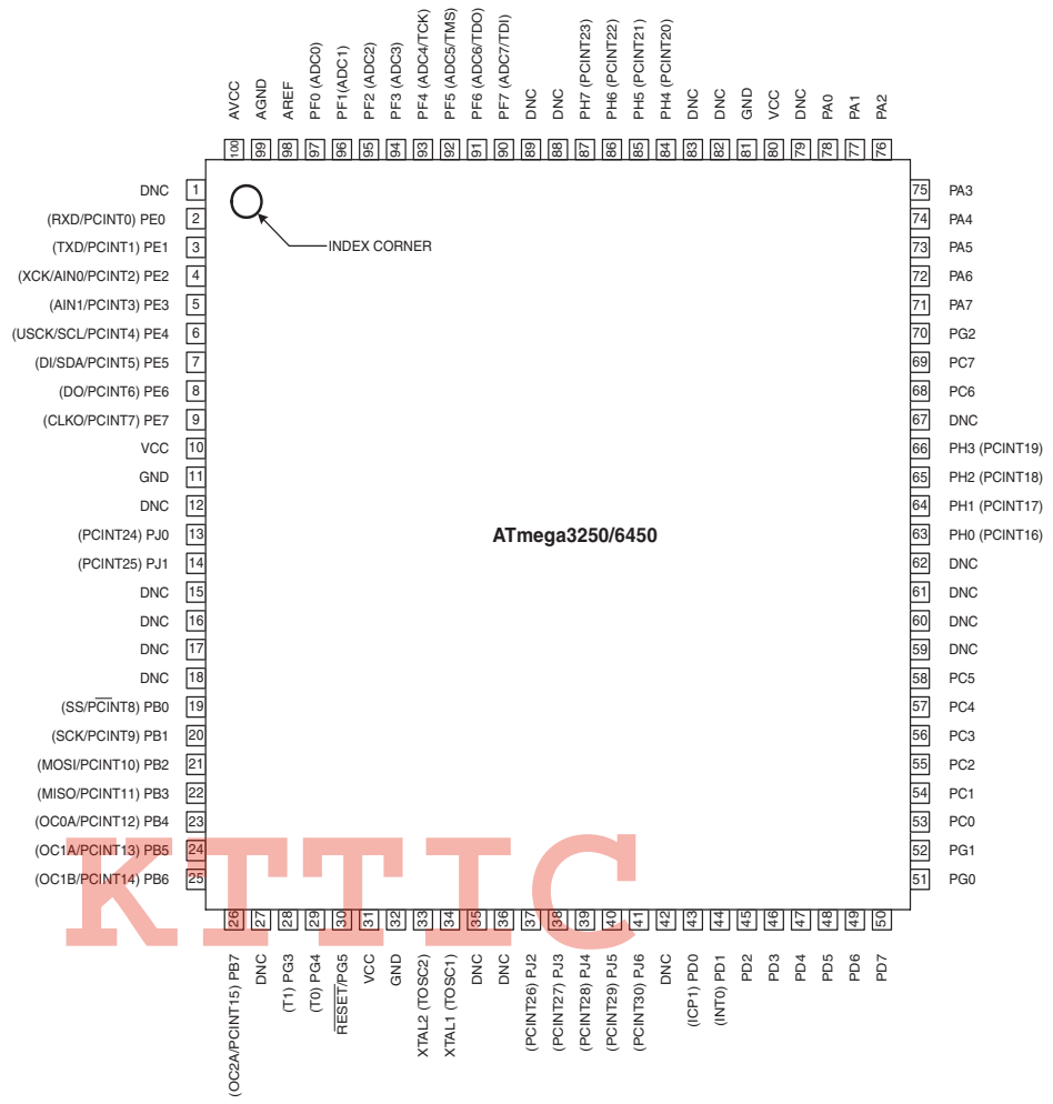
Figure 1-1. Pinout ATmega3250/6450
