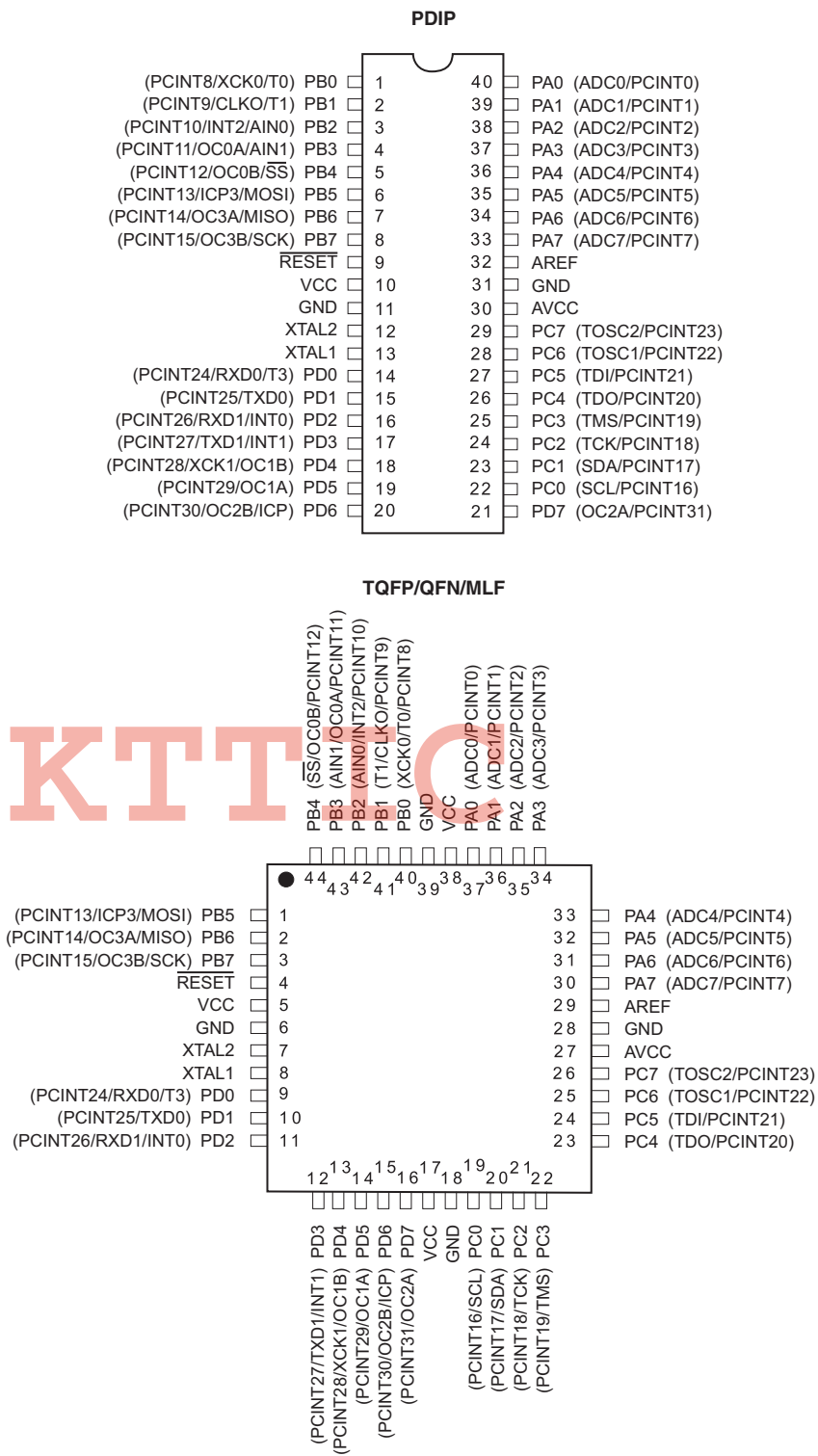
Figure 1-1. Pinout ATmega1284P
