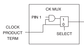
Figure 9-1. Clock Option
