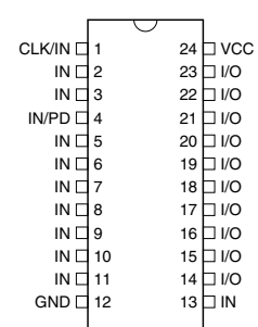
Figure 2-2. DIP/SOIC
