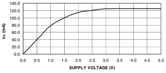
ATF22V10C/CQ OUTPUT SINK CURRENT VS. SUPPLY VOLTAGE ( V_{OL} = 0.5\text{V} )
