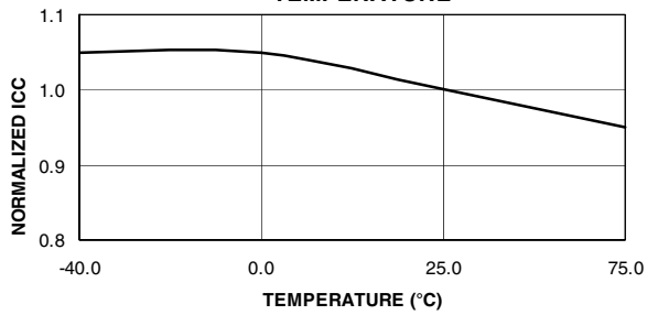
ATF22V10C/CQ NORMALIZED I_{CC} VS. TEMPERATURE
