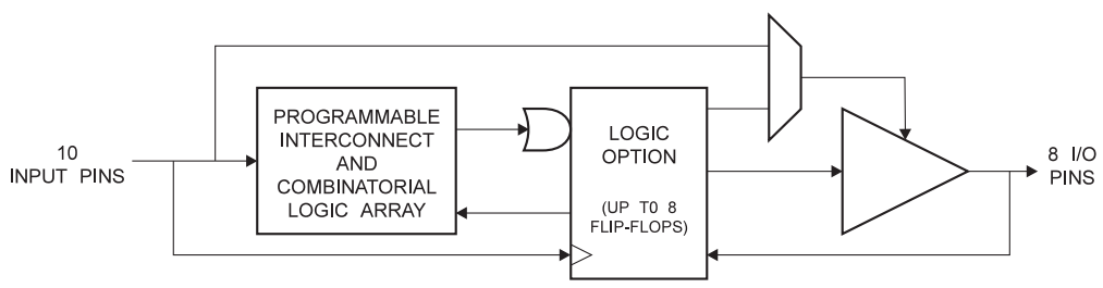
Figure 1-1. Block Diagram
