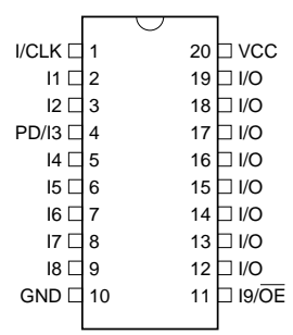
DIP/SOIC
