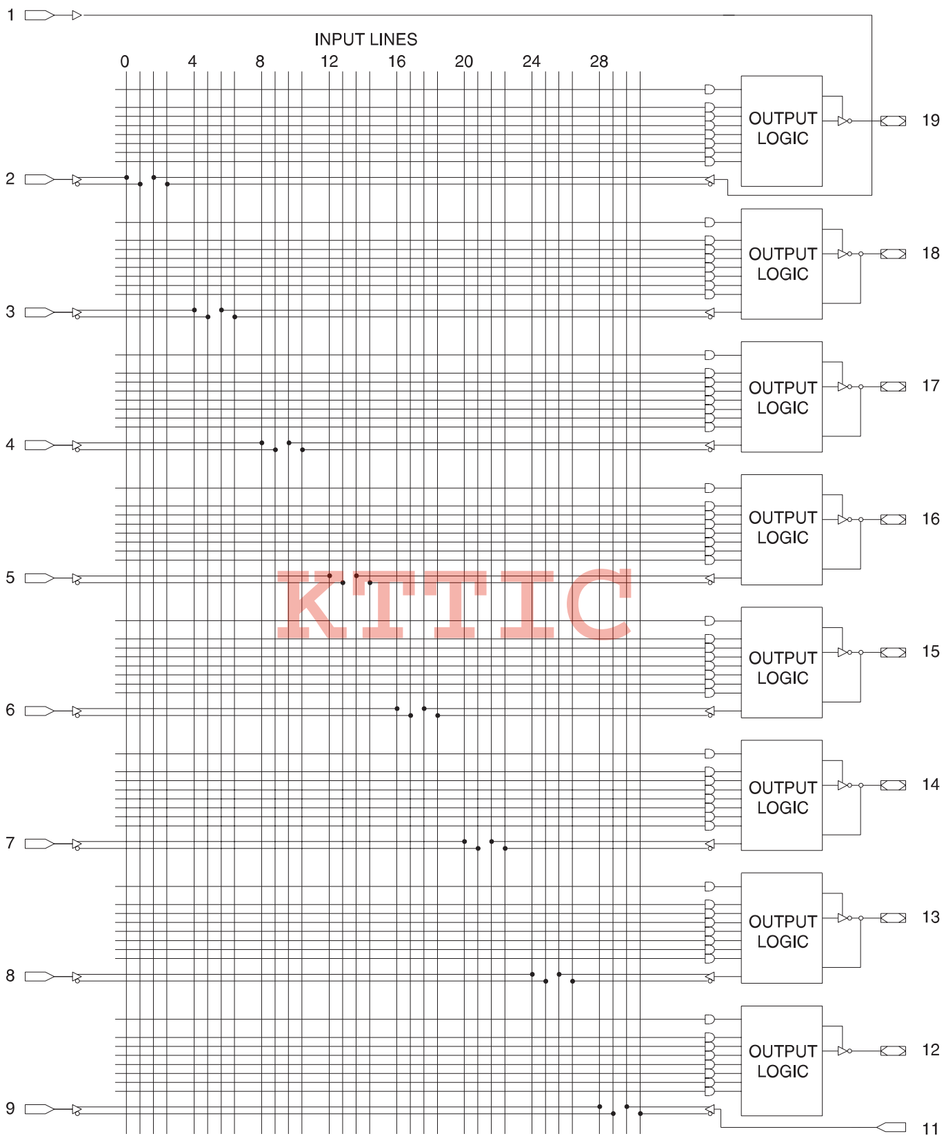
Figure 11-5. Complex Mode Logic Diagram
