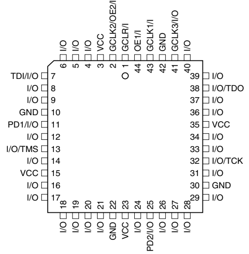
Figure 1-2. 44-lead PLCC Top View
