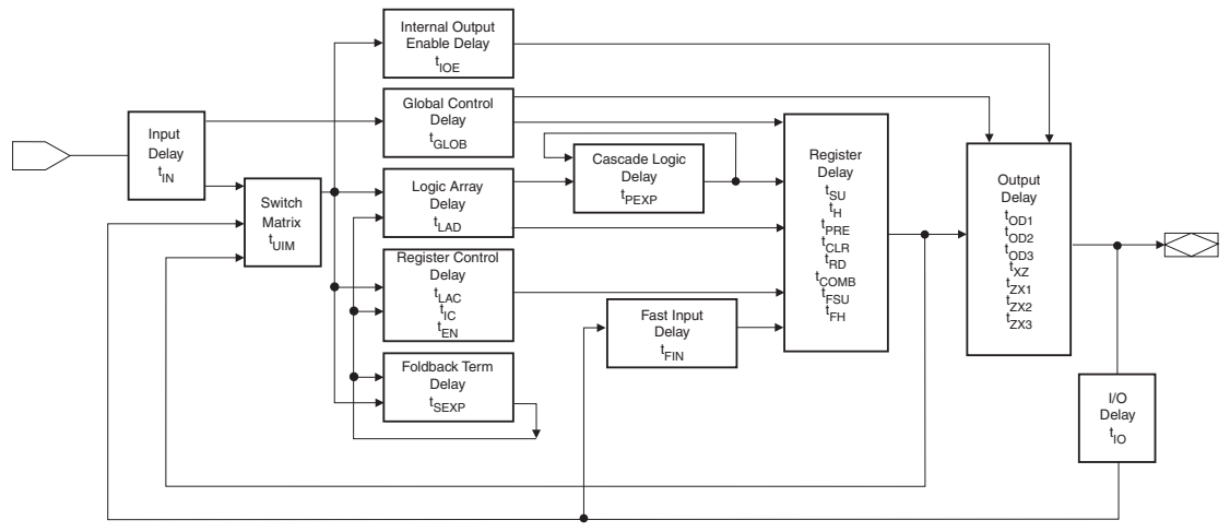
Figure 10-1. Timing Model
