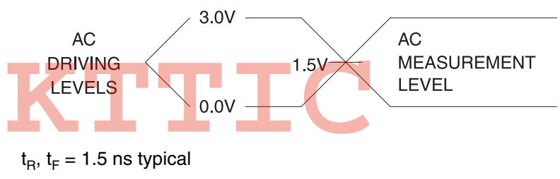
Figure 11-1. Input Test Waveforms and Measurement Levels
