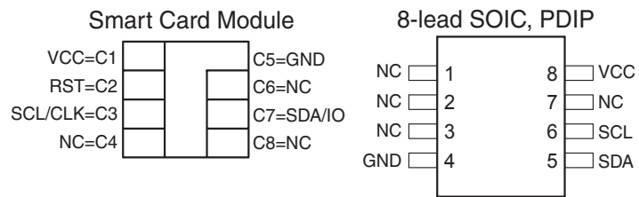
Figure 1. Package Options
