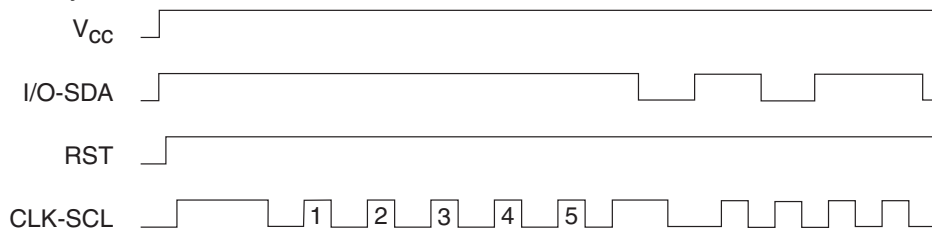
Figure 11. Synchronous 2-wire Protocol
