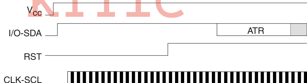
Figure 10. Asynchronous T = 0 Protocol (Gemplus Patent)
