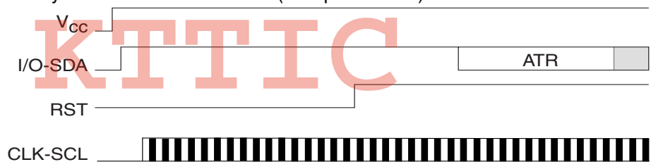
Figure 10. Asynchronous T = 0 Protocol (Gemplus Patent)
