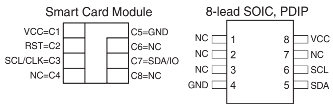
Figure 1. Package Options
