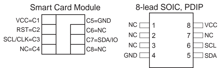
Figure 1. Package Options
