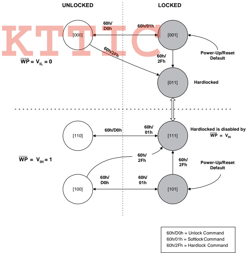
Figure 4-1. Sector Locking State Diagram
