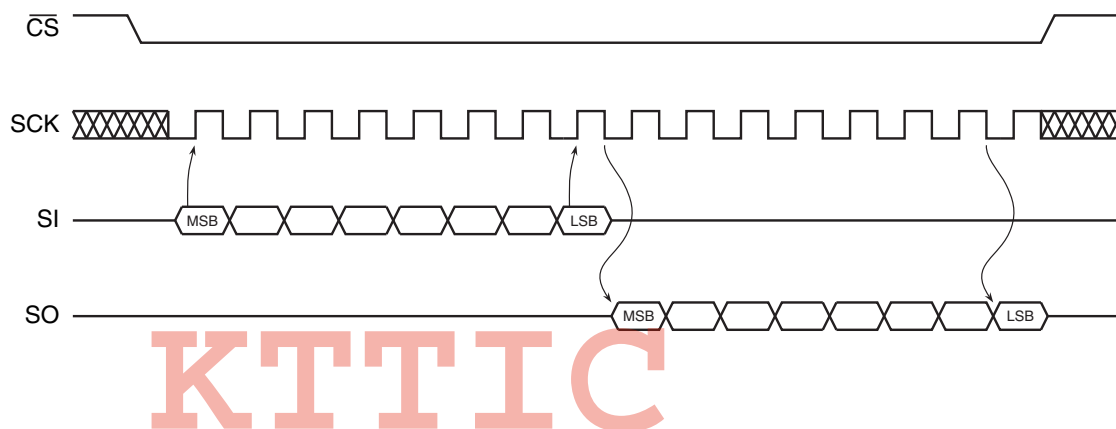
Figure 5-1. SPI Mode 0 and 3
