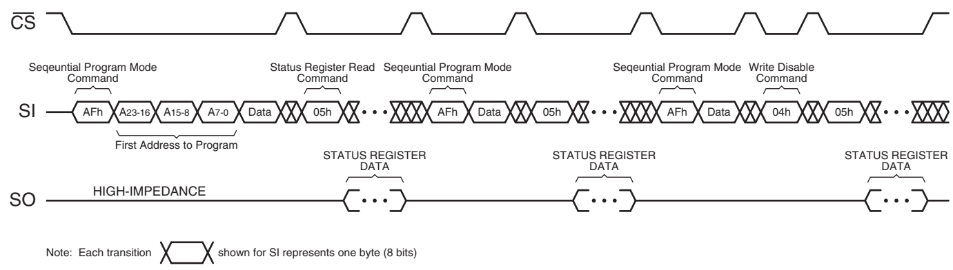
Figure 8-2. Sequential Byte Program Mode – Status Register Polling
