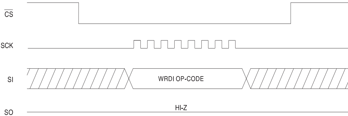
Figure 4-3. WRDI Timing
