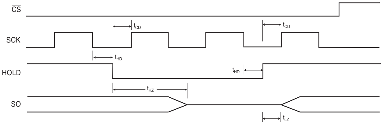
Figure 4-8. HOLD Timing
