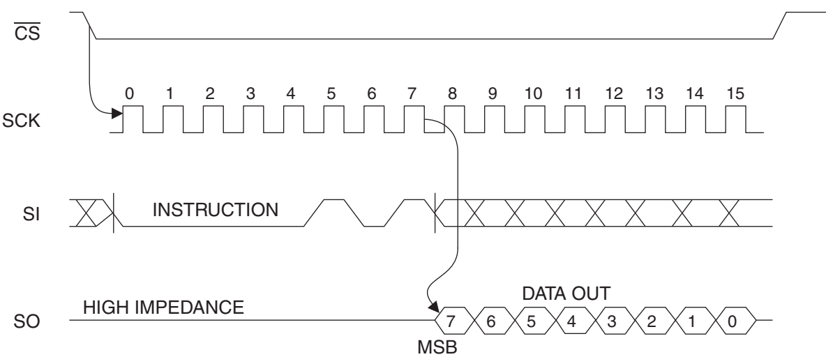
Figure 3-4. RDSR Timing
