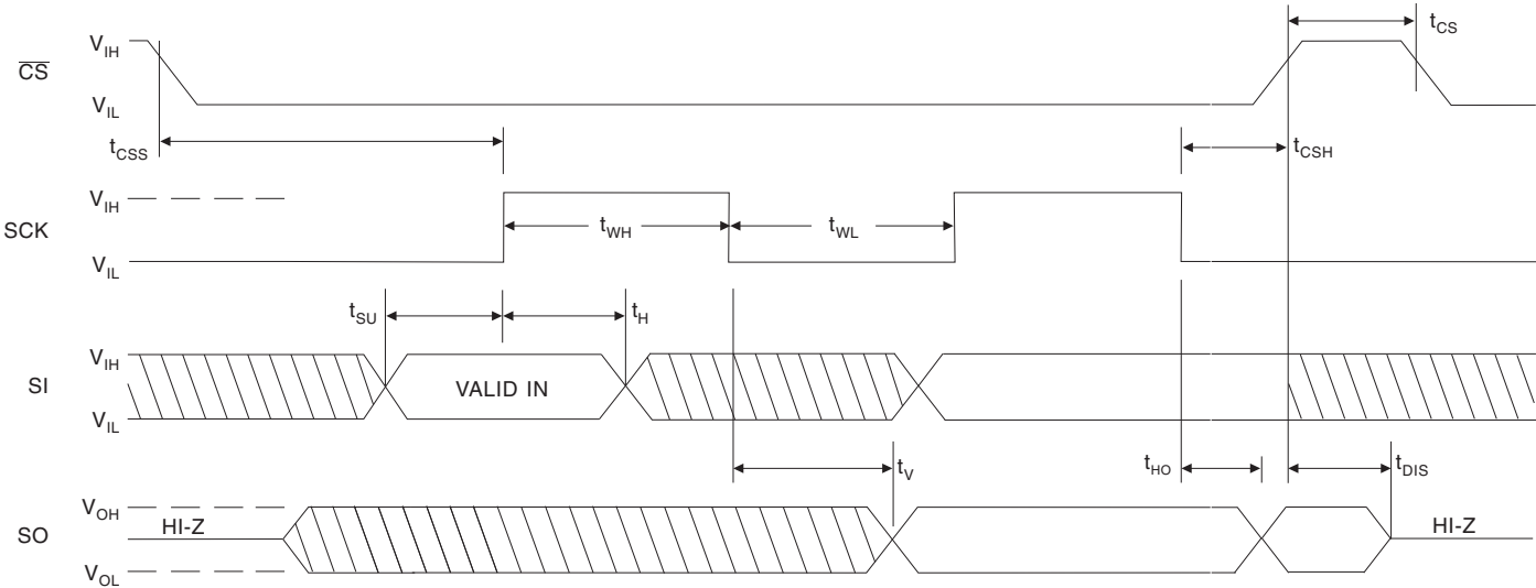
Figure 3-1. Synchronous Data Timing (for Mode 0)
