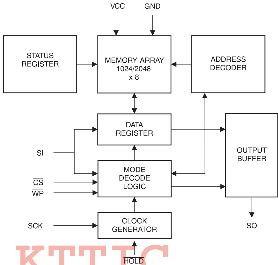
Figure 0-1. Block Diagram
