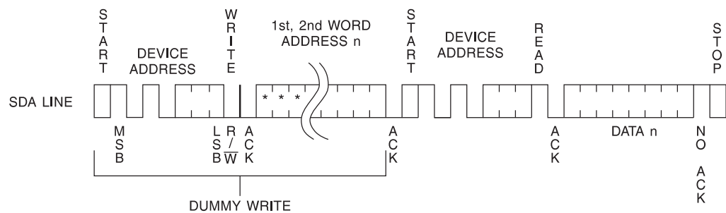
Figure 13-5. Random Read
