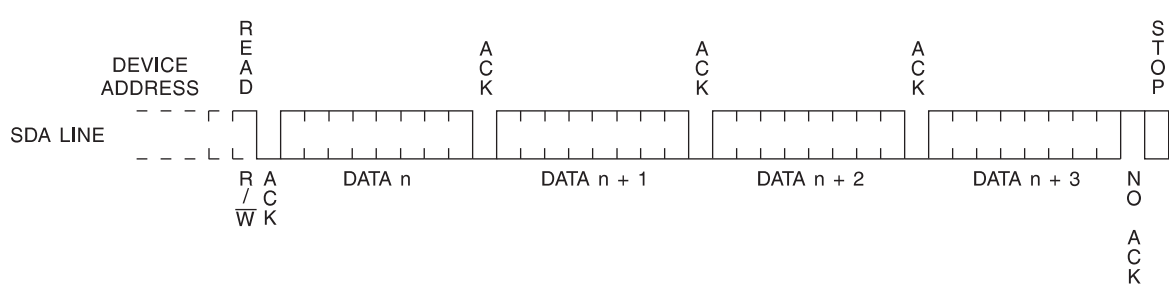
Figure 13-6. Sequential Read
