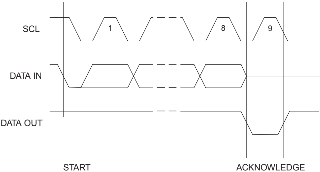
Figure 7. Output Acknowledge
