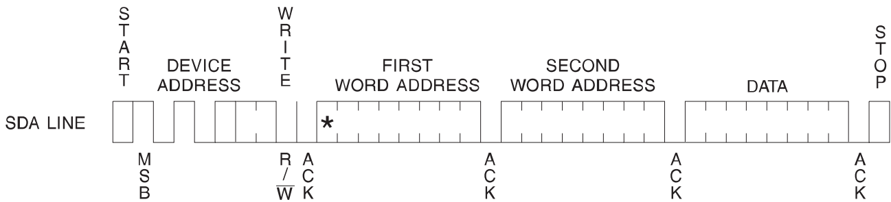
Figure 9. Byte Write
