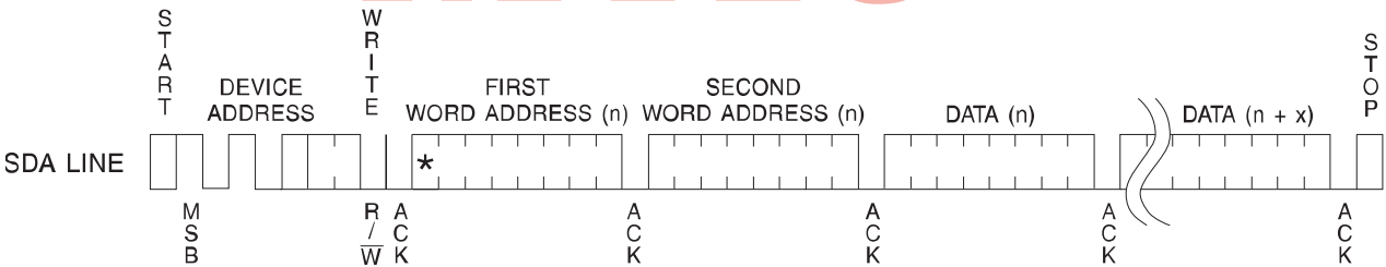
Figure 10. Page Write
