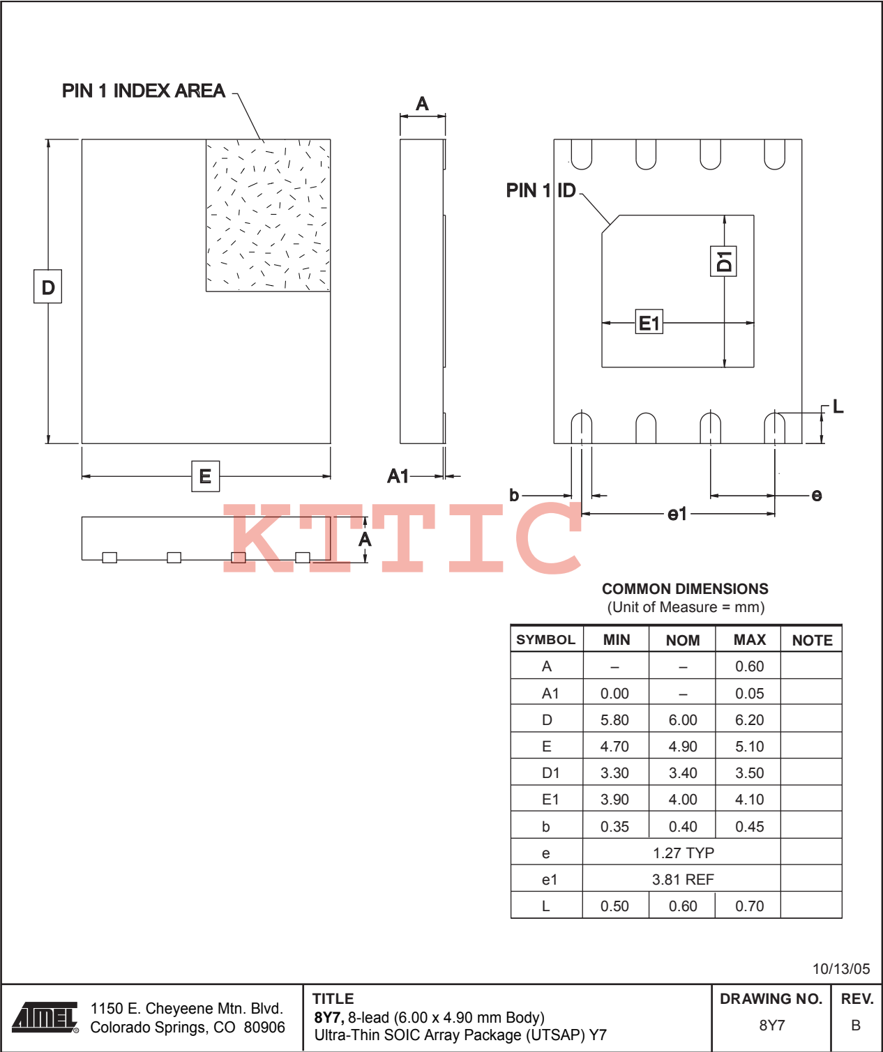
Figure 17. 8Y7 – SAP
