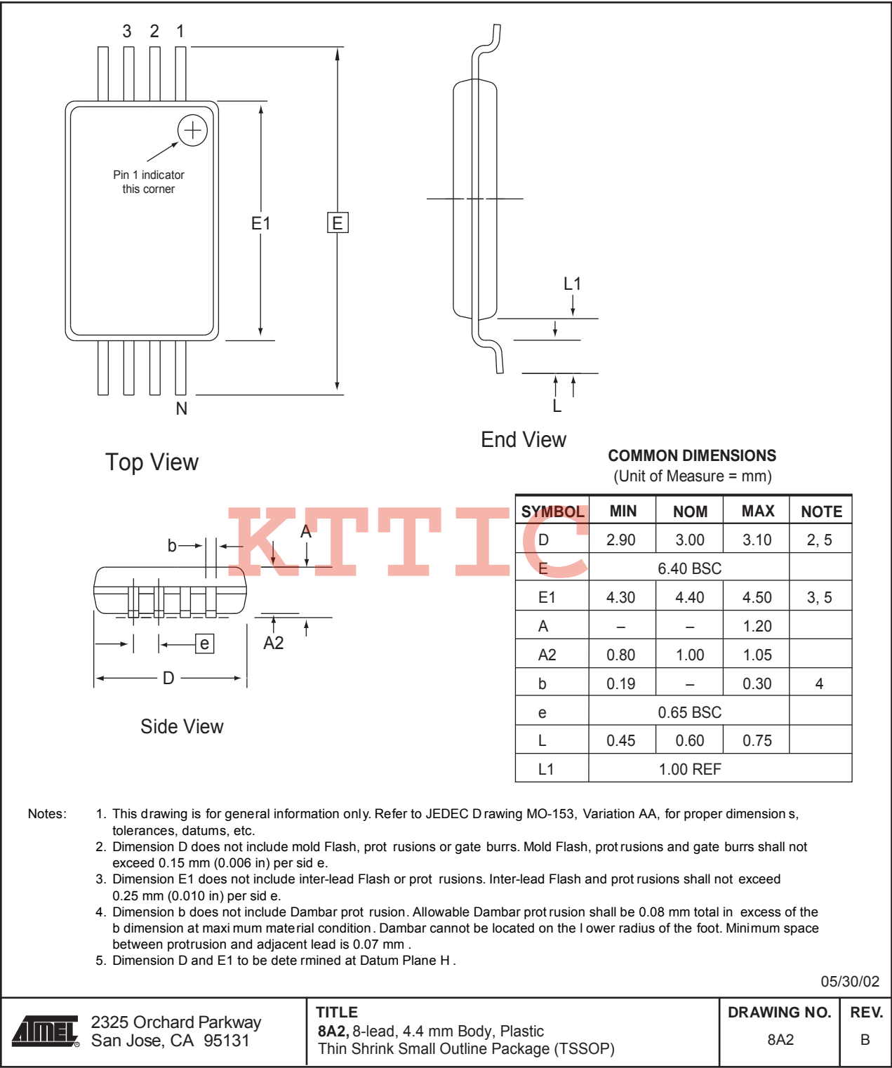
Figure 16. 8A2 – TSSOP
