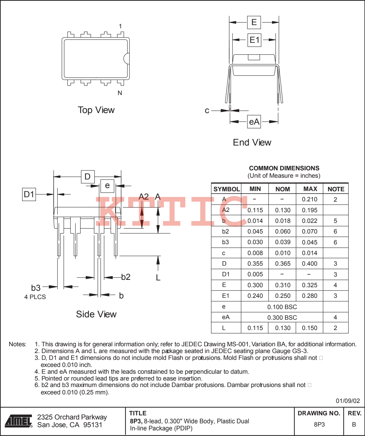
Figure 1. 8P3 – PDIP
