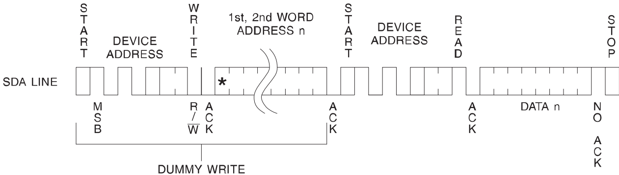
Figure 12. Random Read
