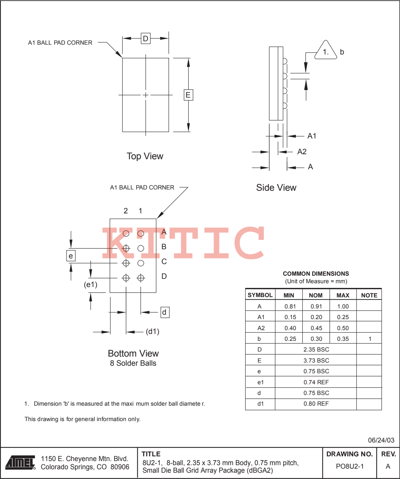
Figure 15. 8U2-1 – dBGA2
