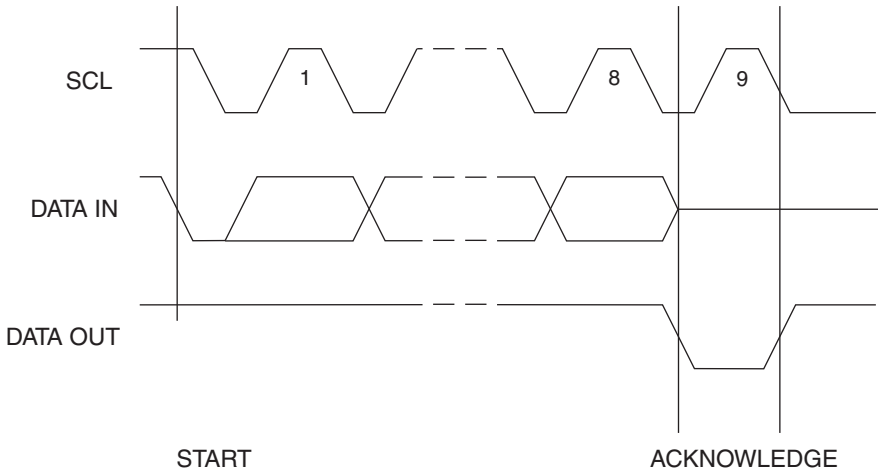
Figure 4-6. Output Acknowledge
