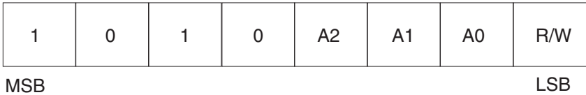
Figure 5-1. Device Address
