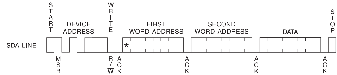
Figure 6-1. Byte Write
