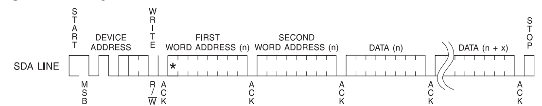
Figure 6-2. Page Write
