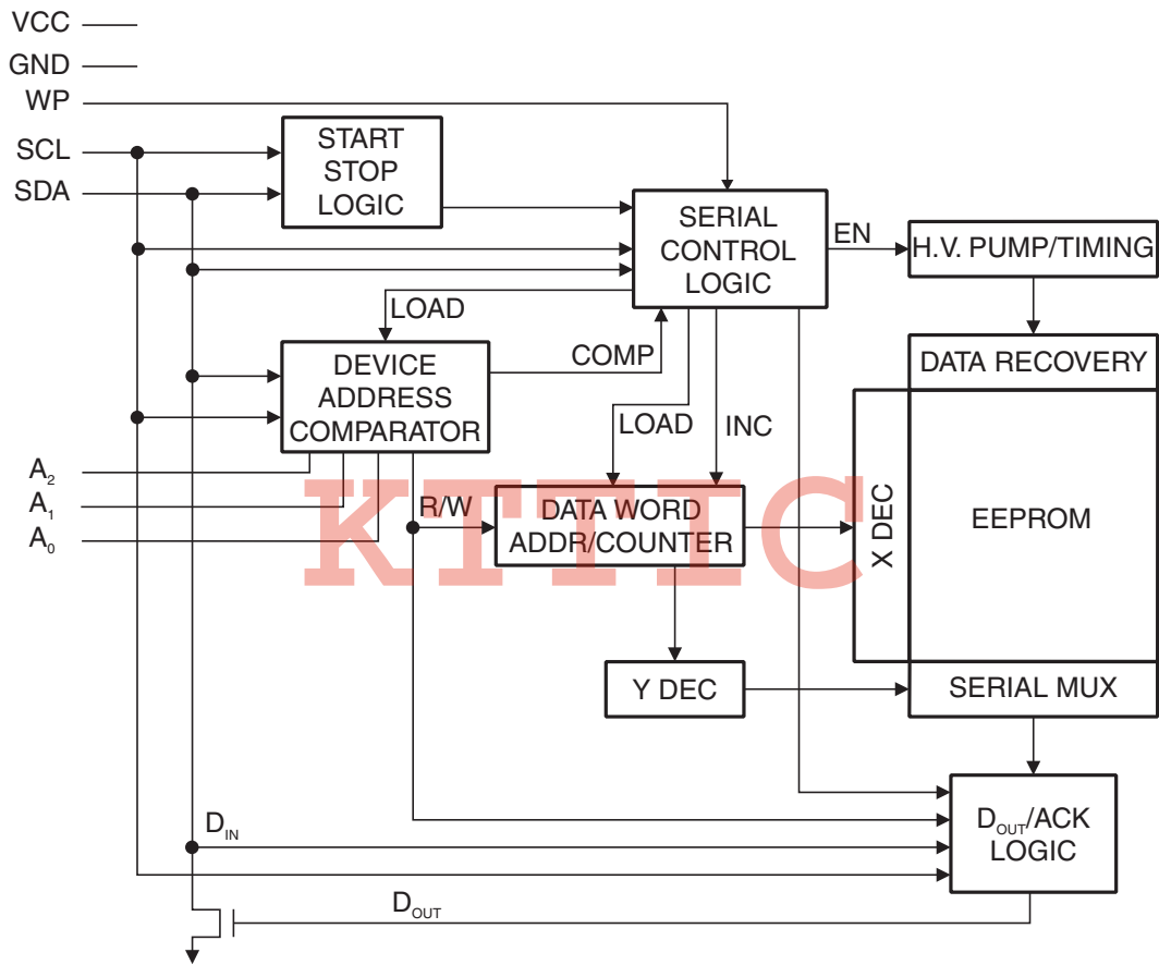
Figure 1-1. Block Diagram
