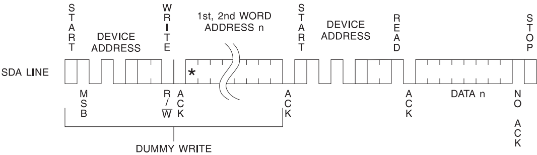
Figure 7-2. Random Read
