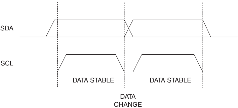
Figure 6. Data Validity
