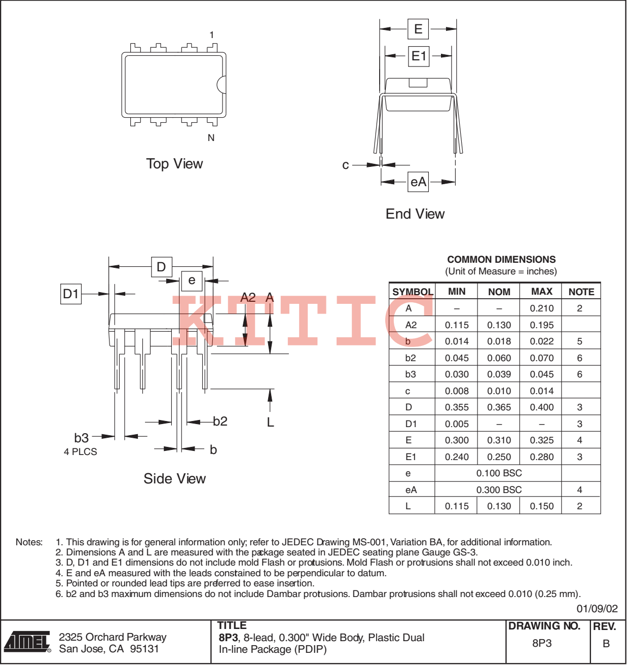
Figure 15. 8P3 – PDIP
