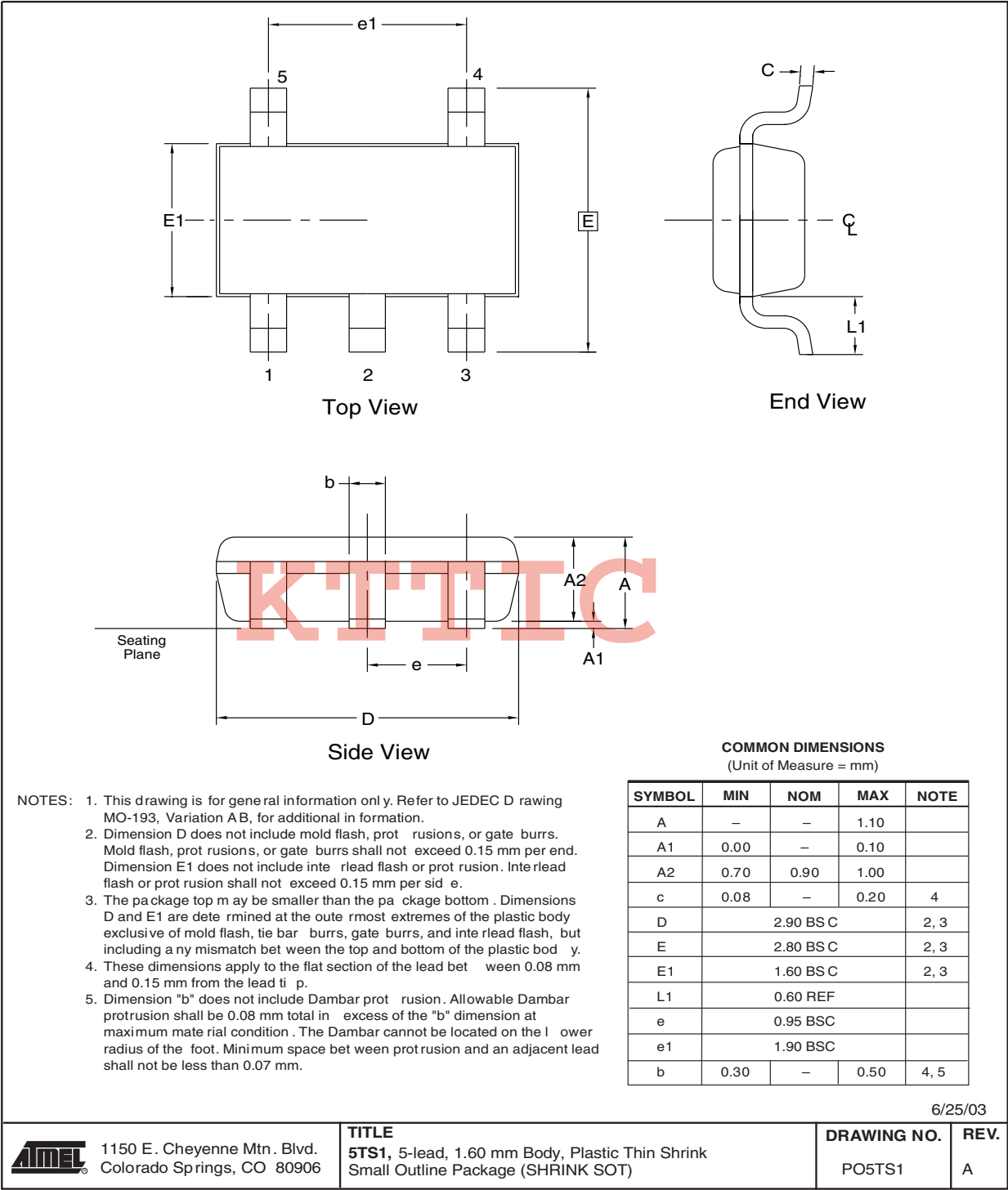
Figure 19. 5TS1 – SOT23
