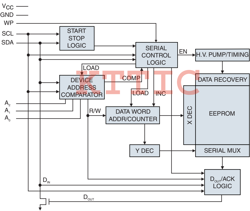
Figure 2. Block Diagram
