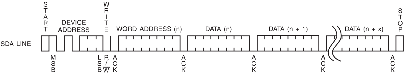
Figure 11. Page Write
