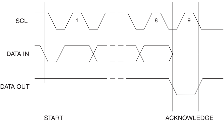
Figure 8. Output Acknowledge
